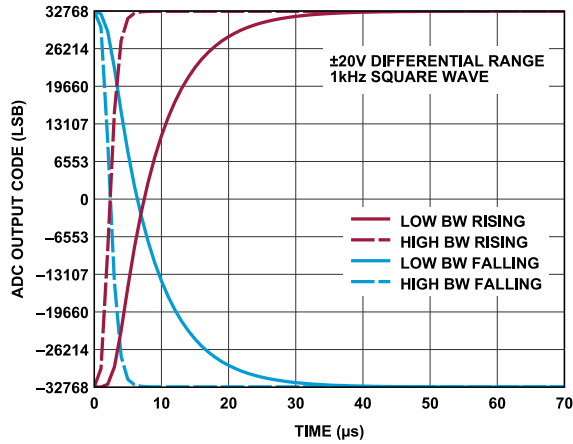
Figure 63. Step Response, \pm 20 V Differential Range
