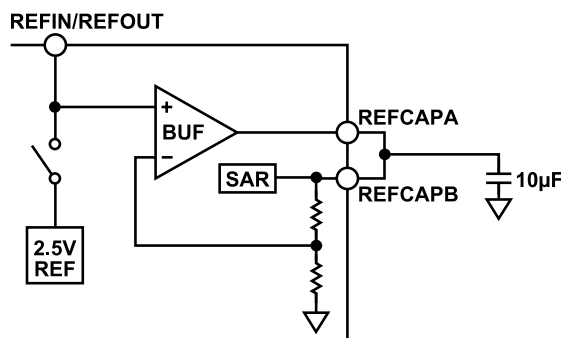
Figure 84. Reference Circuitry
