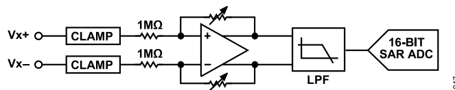
Figure 75. Analog Input Circuitry for Each Channel
