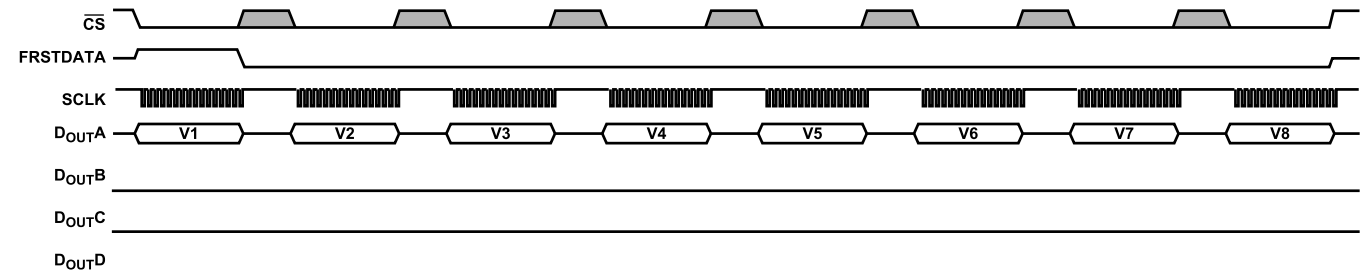
Figure 108. Serial Interface ADC Reading, One D_{OUTX} Lines
