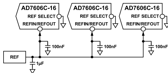
Figure 86. Single External Reference Driving Multiple AD7606C-16 REF \overline{\text{OUT}} Pins
