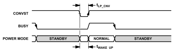
Figure 87. Autostandby Mode Operation
