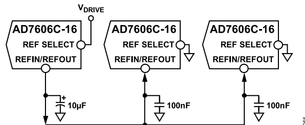
Figure 85. Internal Reference Driving Multiple AD7606C-16 REF \overline{\text{OUT}} Pins
