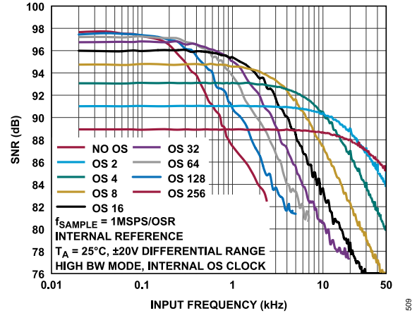
Figure 18. SNR vs. Input Frequency for Different OSR Values, ±20 V Differential Range, High Bandwidth Mode, Internal Oversampling Clock
