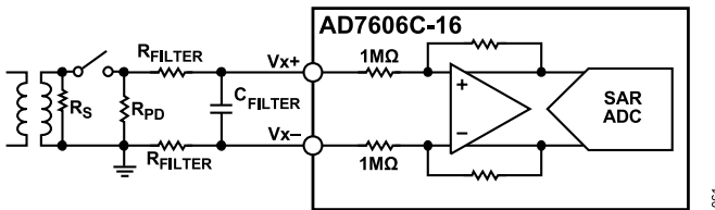
Figure 96. Analog Front End with R_{PD}
