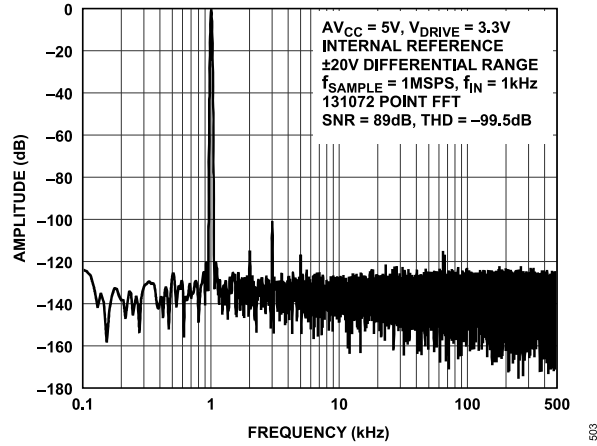
Figure 12. FFT, ±20 V Differential Range, High Bandwidth Mode
