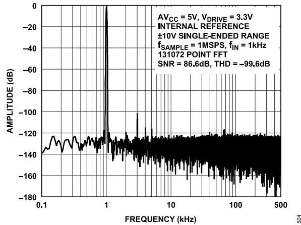
Figure 13. FFT, ±10 V Single-Ended Range, High Bandwidth Mode
