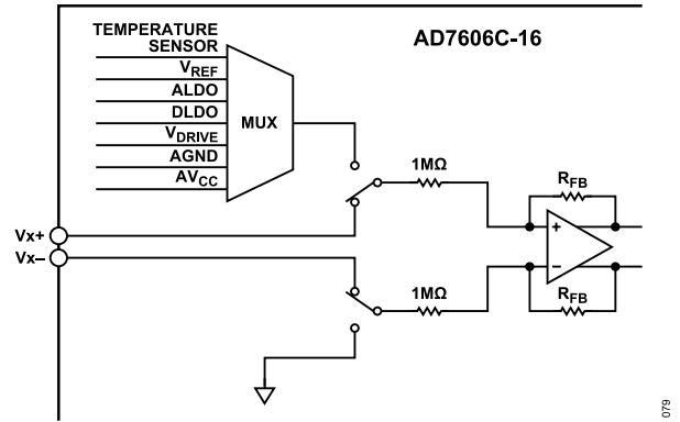
Figure 118. Diagnostic Multiplexer (Channel 1 Shown as an Example) (R FB = Feedback Resistor)
