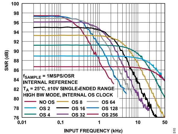
Figure 19. SNR vs. Input Frequency for Different OSR Values, ±10 V Single-Ended Range, High Bandwidth Mode, Internal Oversampling Clock
