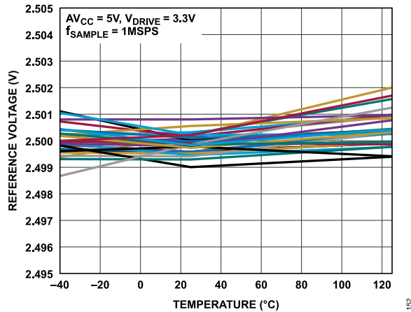
Figure 61. Reference Drift
