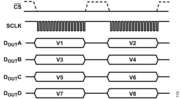
Figure 106. Serial Interface ADC Reading, Four D_{OUTX} Lines
