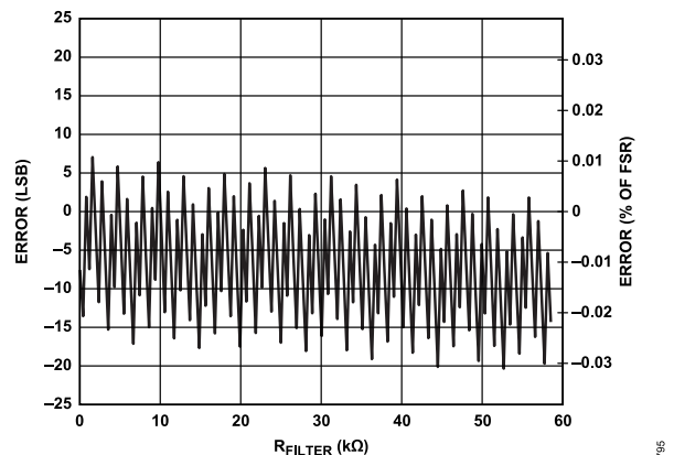
Figure 95. System Error with Gain Calibration Enabled
