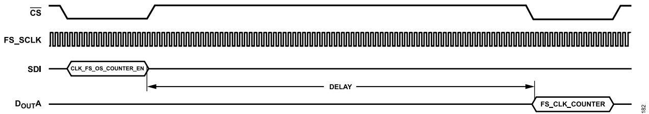
Figure 120. FS_CLK_COUNTER Functionality
