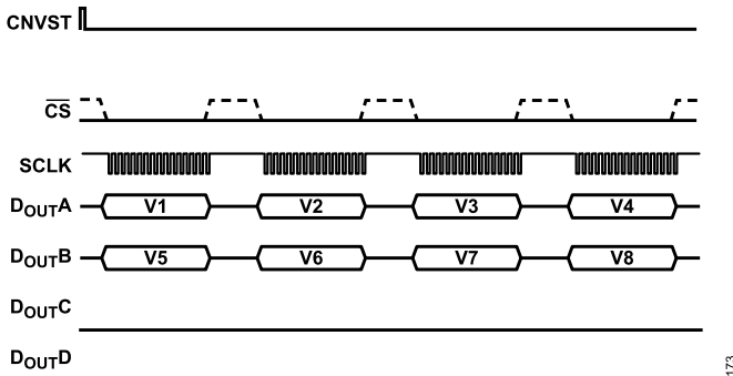
Figure 105. Serial Interface ADC Reading, Two D_{OUTX} Lines
