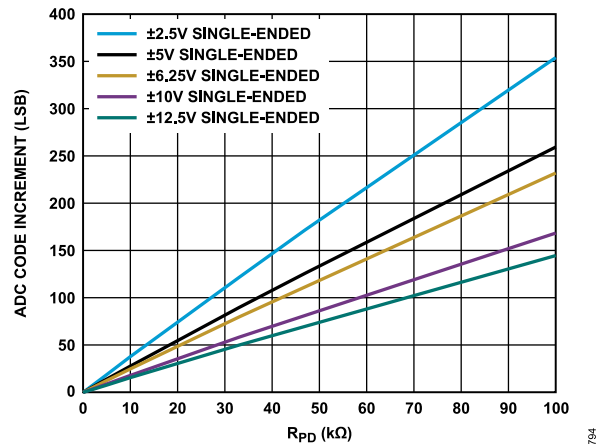
Figure 97. Open Circuit Code Error Increment, Dependent of R_{PD}
