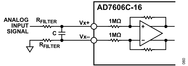
Figure 93. System Gain Error
