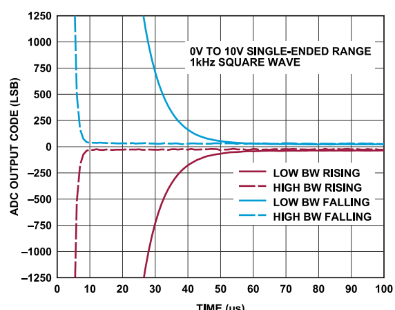
Figure 68. Step Response, 0 V to 10 V Single-Ended Range, Fine Settling
