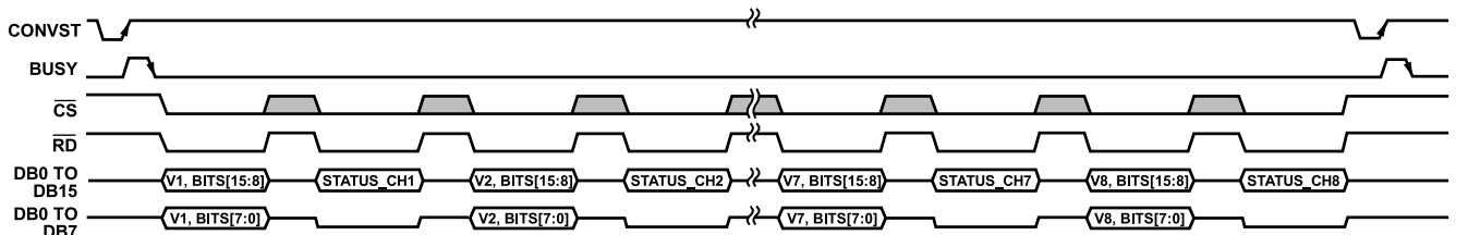
Figure 100. Parallel Interface, ADC Mode with Status Header Enabled
