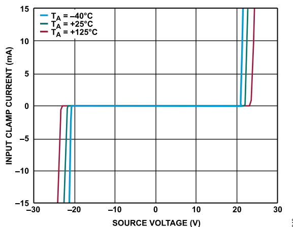
Figure 76. Input Protection Clamp Profile
