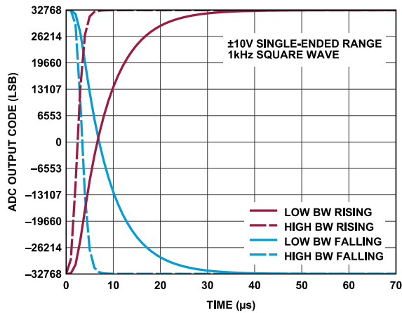
Figure 64. Step Response, \pm 10 V Single-Ended Range
