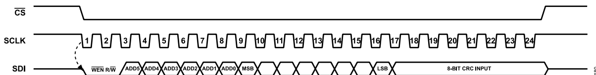
Figure 115. Writing Registers Through the SPI Interface with CRC Enabled
