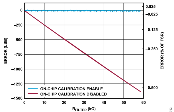
Figure 94. System Gain Calibration with and Without Calibration, \pm 10 V Single-Ended Range
