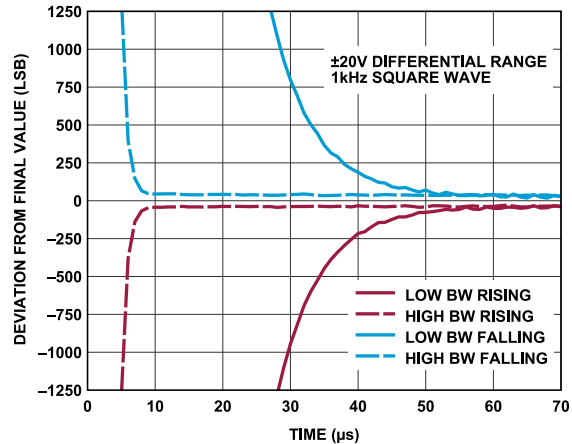
Figure 66. Step Response, \pm 20 V Differential Range, Fine Settling
