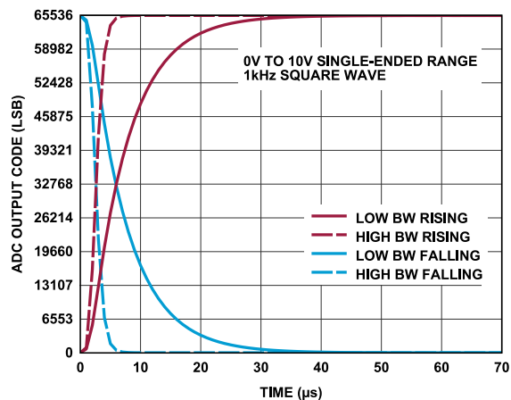
Figure 65. Step Response, 0 V to 10 V Single-Ended Range
