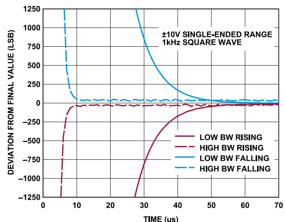
Figure 67. Step Response, \pm 10 V Single-Ended Range, Fine Settling
