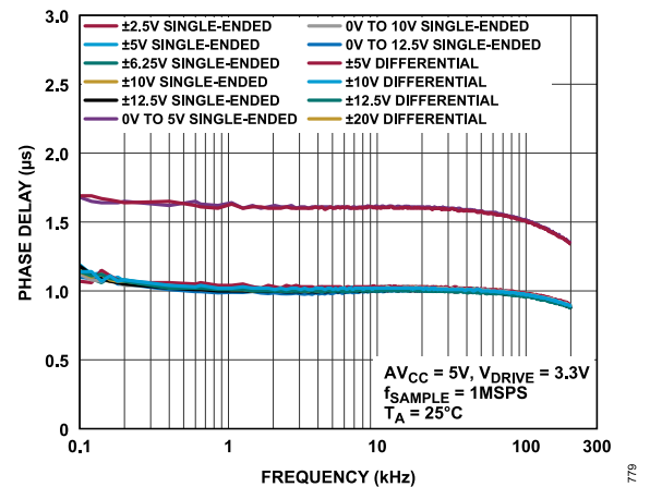
Figure 81. Analog Antialiasing Filter Phase Response, High Bandwidth Mode
