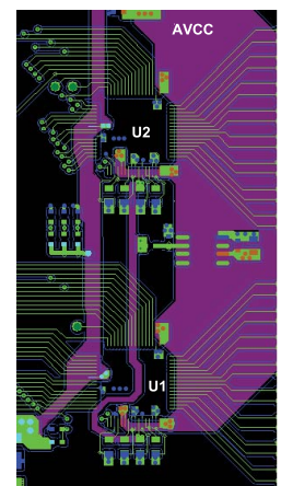
Figure 126. Layout for Multiple AD7606C-16 Devices—Top Layer and Supply Plane Layer
