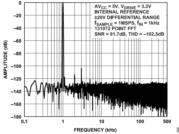
Figure 9. Fast Fourier Transform (FFT), ±20 V Range, Low Bandwidth Mode
