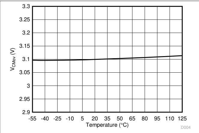
图 7-6. Common-Mode Overvoltage Detection Level vs Temperature
