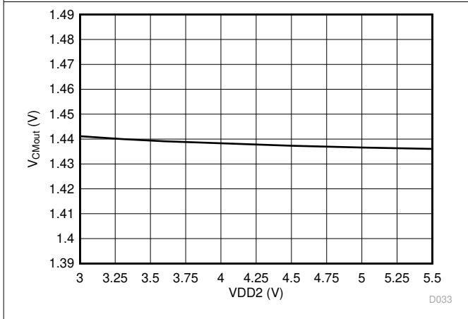
图 7-31. Output Common-Mode Voltage vs Low-Side Supply Voltage
