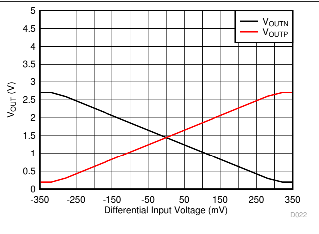
图 7-20. Output Voltage vs Input Voltage
