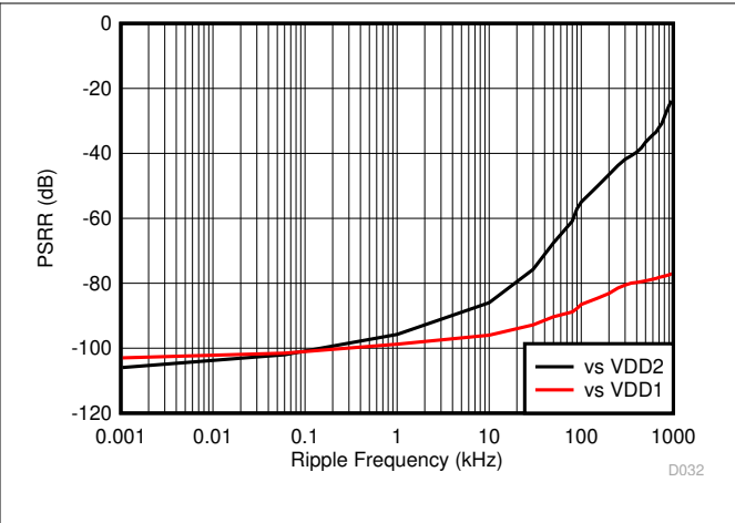
图 7-30. Power-Supply Rejection Ratio vs Ripple Frequency
