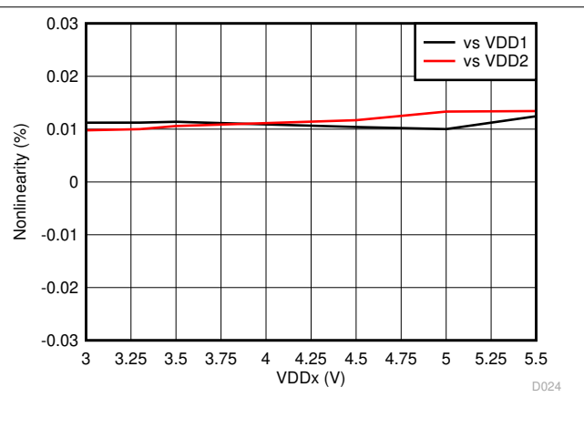
图 7-22. Nonlinearity vs Supply Voltage
