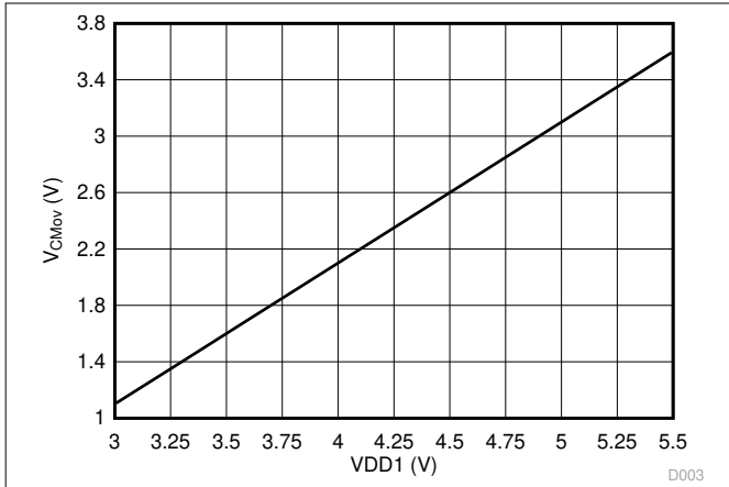
图 7-5. Common-Mode Overvoltage Detection Level vs High-Side Supply Voltage
