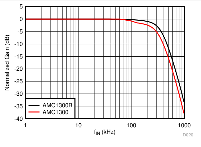
图 7-18. Normalized Gain vs Input Frequency
