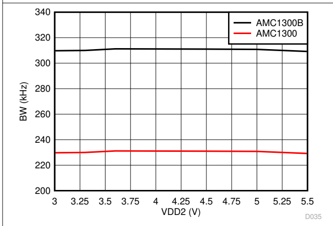
图 7-33. Output Bandwidth vs Low-Side Supply Voltage
